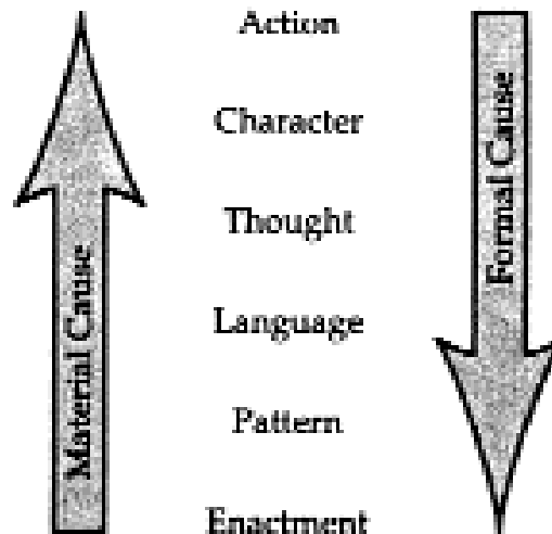
Figure 38.1. Causal relations among elements of quantitative structure.
